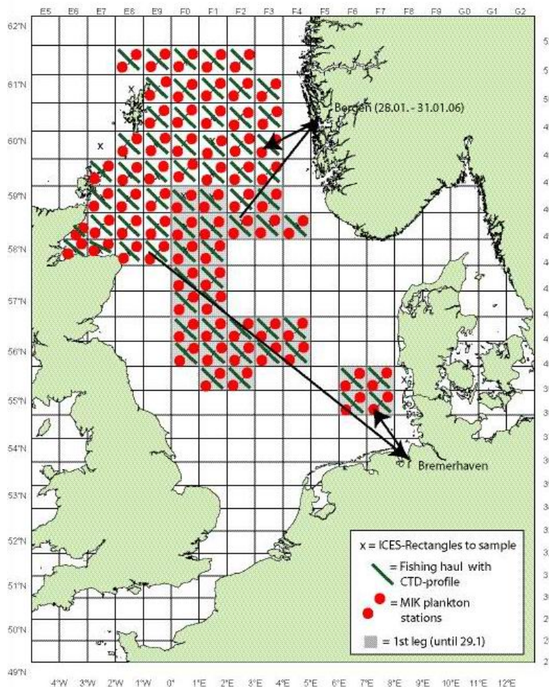
Fig. 7.4: International Bottom Trawl Survey (IBTS) 1 st quarter. MIK and fishery stations of the 2006 survey as an example for the study area.
