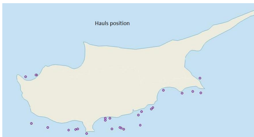
Figure III.G.1. Distribution of sampling hauls of the 2016 Medits survey
